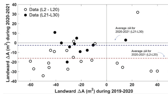
Figure 9. Comparison between landward \Delta A during 2019–2020 and 2020–2021 with a small \Delta A for L21-L30 during 2020–2021.
