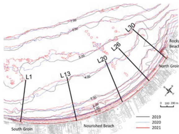
Figure 4. Depth contours in meters surveyed in February 2019, February 2020, and January 2021.
