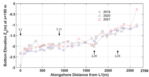
Figure 7. Bottom elevation Z_b at x = 100 m along L1-L30 during 2019-2021.
