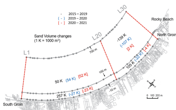
Figure 12. Sand volume changes in landward and seaward zones during 2015–2019 in comparison with those changes (in parentheses) during 2019–2020, and (brackets) during 2020–2021, where points (solid circles) along each of L1–L30 are located at the offshore distances of -10, 100, and 700 m.
