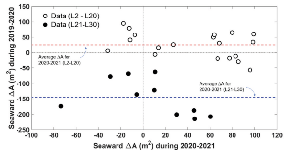
Figure 11. Comparison between seaward \Delta A during 2019–2020 and 2020-2021.
