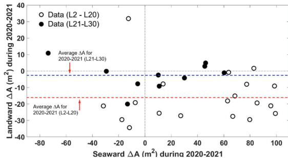
Figure 10. Comparison between seaward \Delta A and landward \Delta A during 2020–2021.
