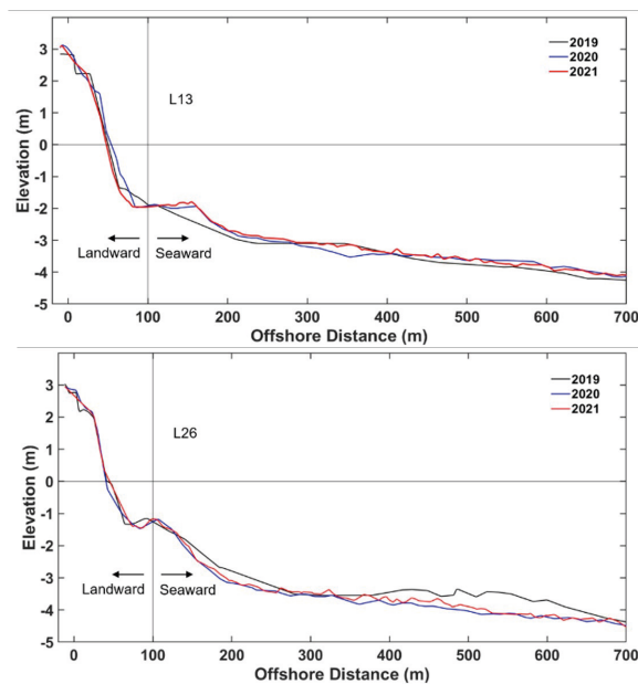
Figure 5. Beach profiles in 2019, 2020, and 2021 along Line L13 with offshore accretion and Line L26 with offshore erosion during 2019-2020.
