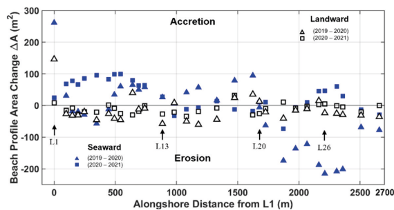
Figure 8. Beach profile area changes \Delta A in landward and seaward zones along L1–L30 during 2019–2020 and 2020–2021.
